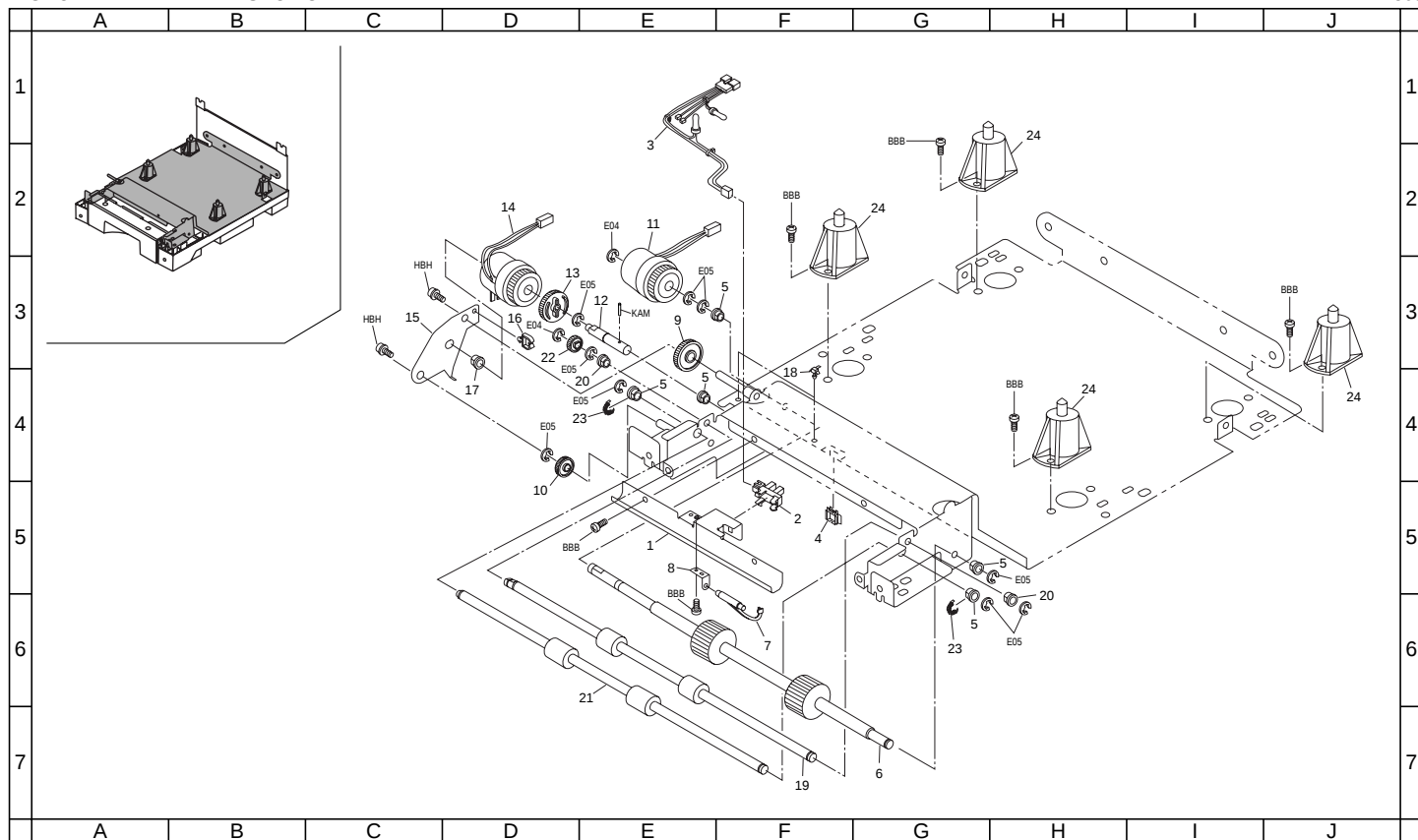
FIG. 3 PAPER FEED-IN SECTION
